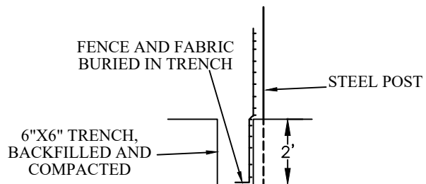
SECTION VIEW AT OPENING
