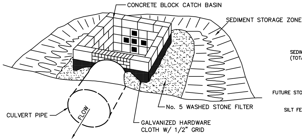
PERSPECTIVE VIEW
