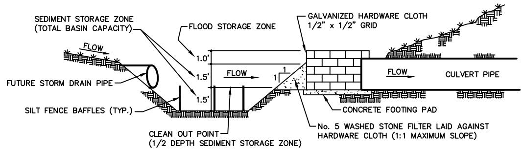
SECTION VIEW
