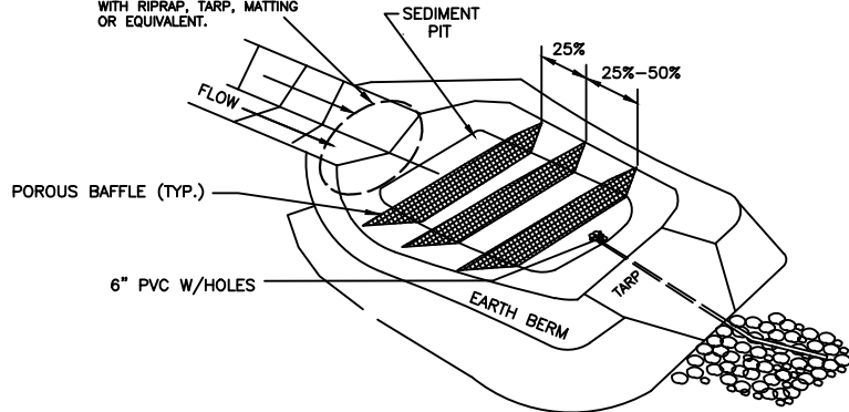
PERSPECTIVE VIEW
