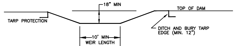
SECTION THRU WEIR
